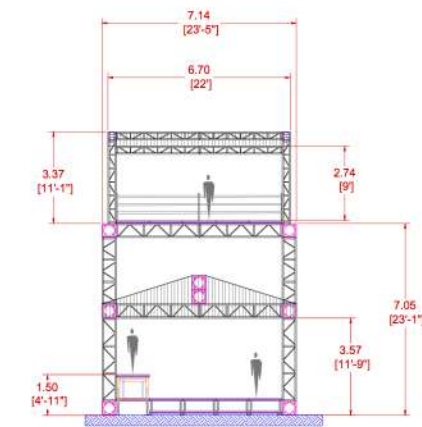
VISTA FRONTAL
