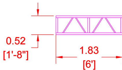
Truss 6 FT
