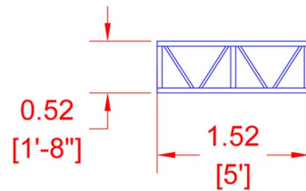
Truss 5 FT
