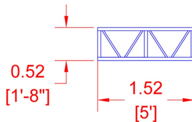
Truss 5 FT
